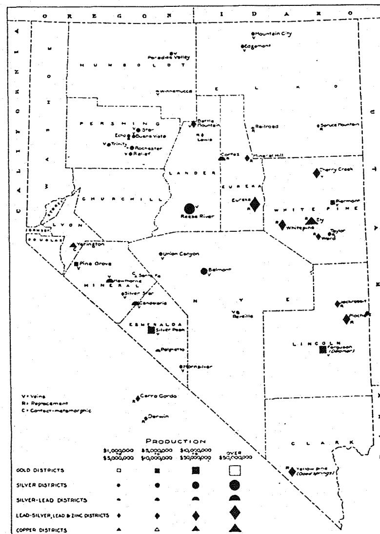
FIGURE 1. Map showing distribution of principal ore deposits in Nevada associated with granitic intrusives.
