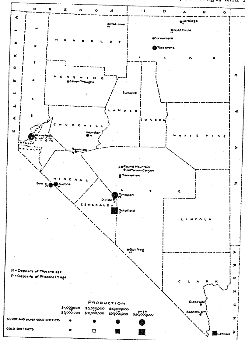
FIGURE 2. Map showing distribution of principal ore deposits in Nevada associated with Tertiary lavas
