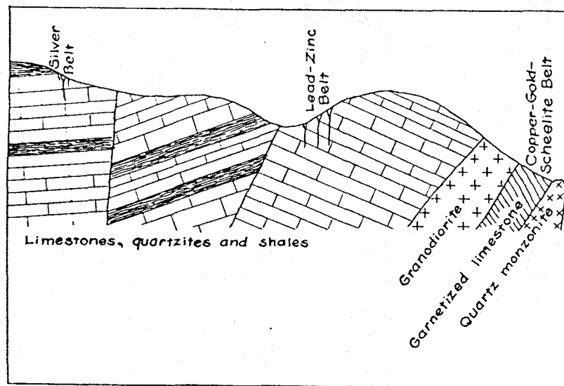
FIGURE 3. East-west section through the White Pine district showing relation of mineral belts to exposed intrusives.*
