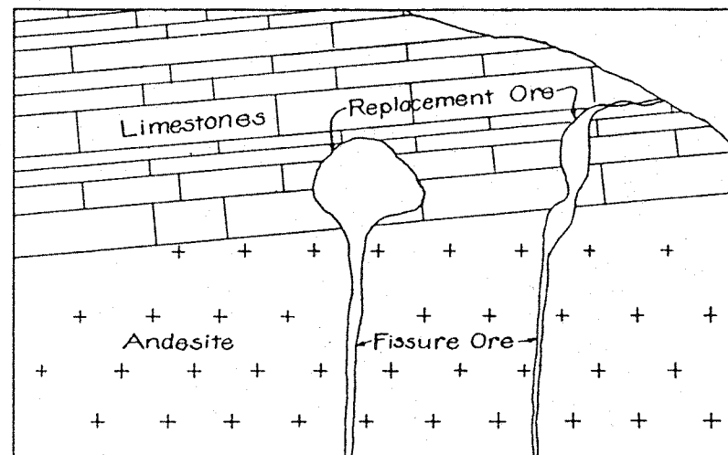
FIGURE 2. East-west vertical cross section through ore bodies of the Queen of Sheba mine, showing relation of replacement ore in limestone to fissure ore in andesite. (This mine was sampled and examined by the writer in December 1934.)
